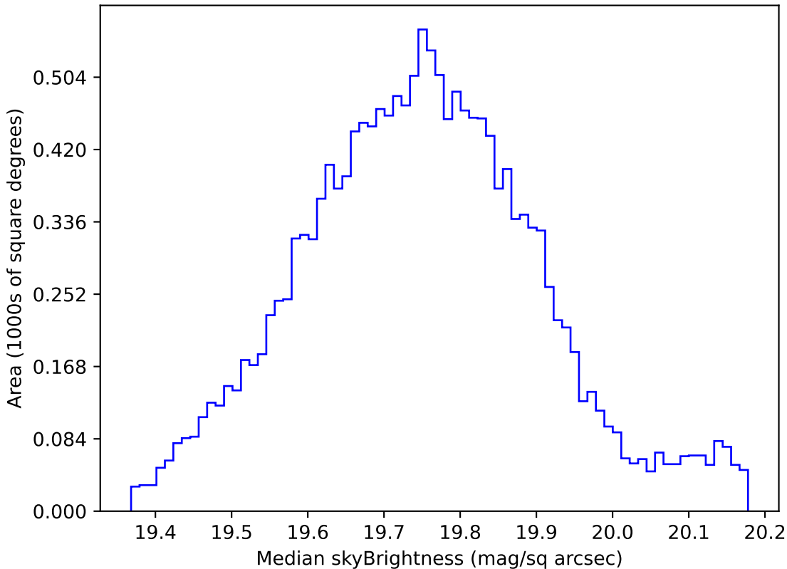
baseline_v3.0_10yrs WFD all bands: Median skyBrightness
