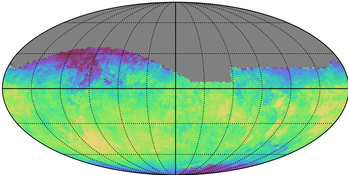
baseline_v3.0_10yrs All sky z band: Median skyBrightness
