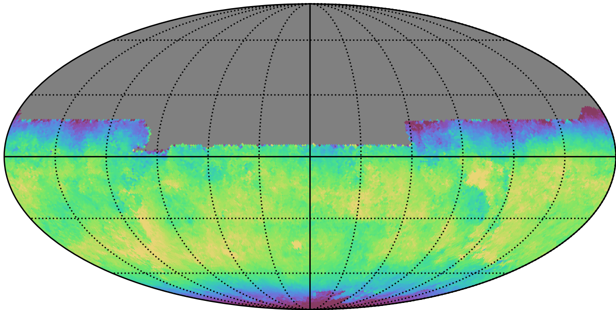
baseline_v3.0_10yrs All sky y band: Median skyBrightness
