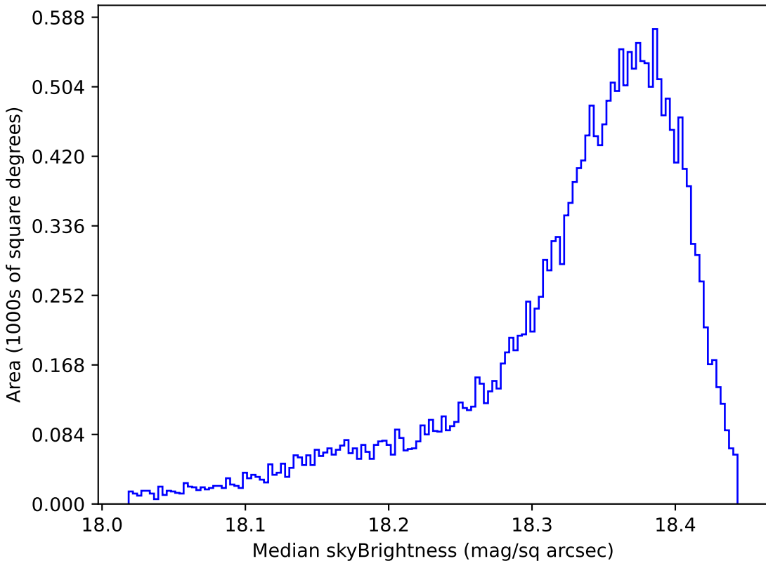
baseline_v3.0_10yrs All sky y band: Median skyBrightness
