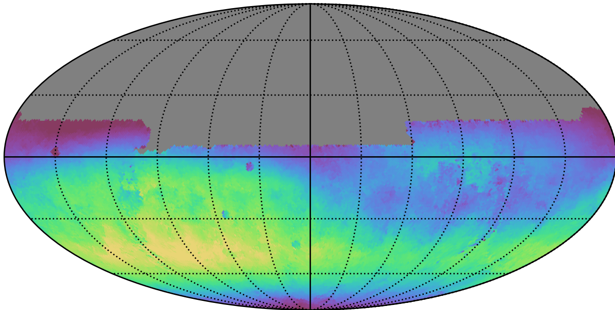
baseline_v3.0_10yrs All sky u band: Median skyBrightness
