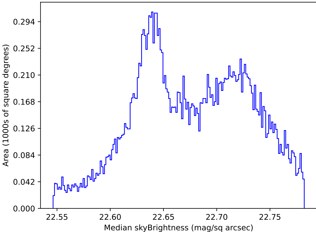
baseline_v3.0_10yrs All sky u band: Median skyBrightness
