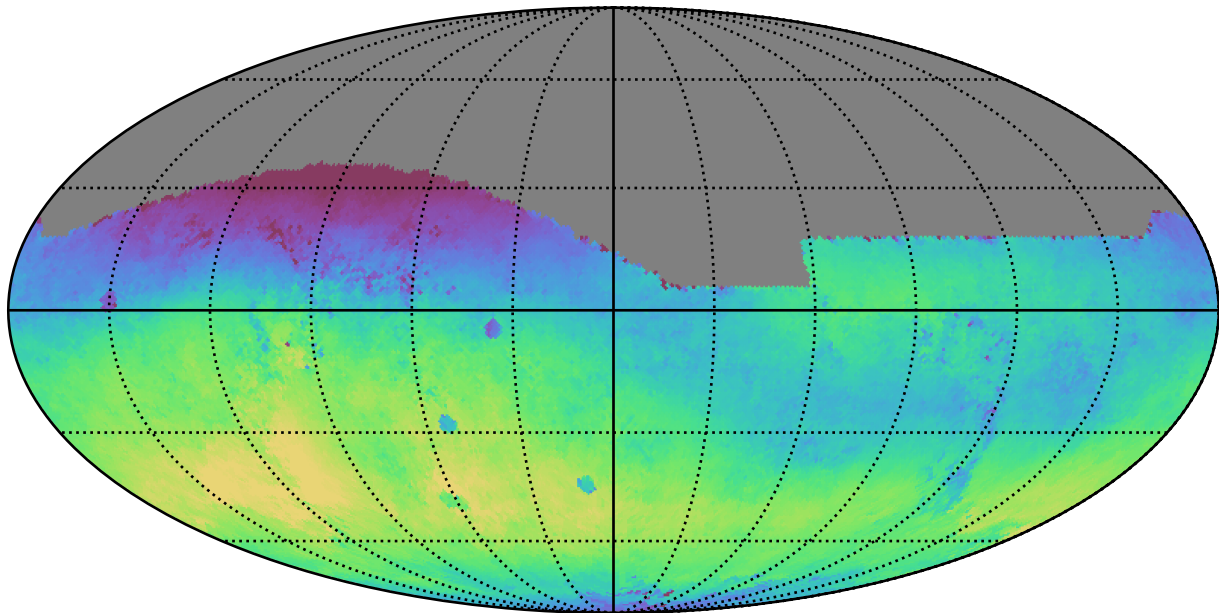
baseline_v3.0_10yrs All sky r band: Median skyBrightness
