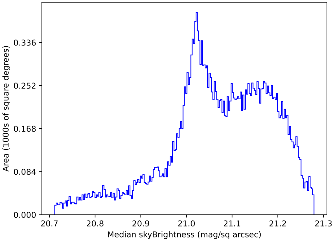
baseline_v3.0_10yrs All sky r band: Median skyBrightness
