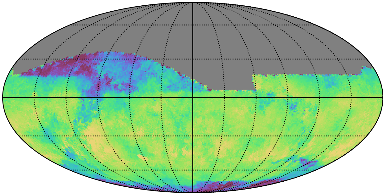
baseline_v3.0_10yrs All sky i band: Median skyBrightness
