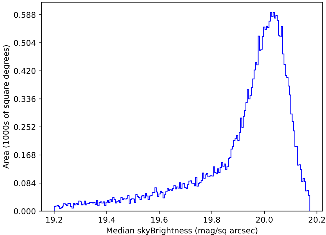
baseline_v3.0_10yrs All sky i band: Median skyBrightness
