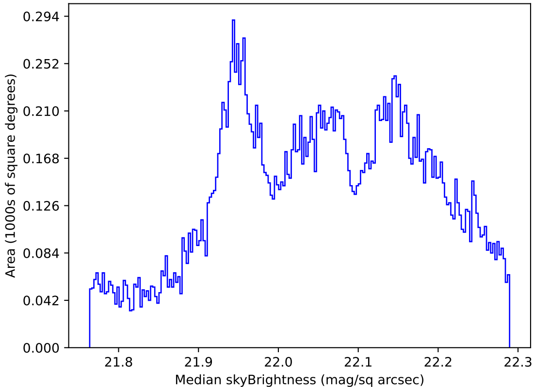
baseline_v3.0_10yrs All sky g band: Median skyBrightness
