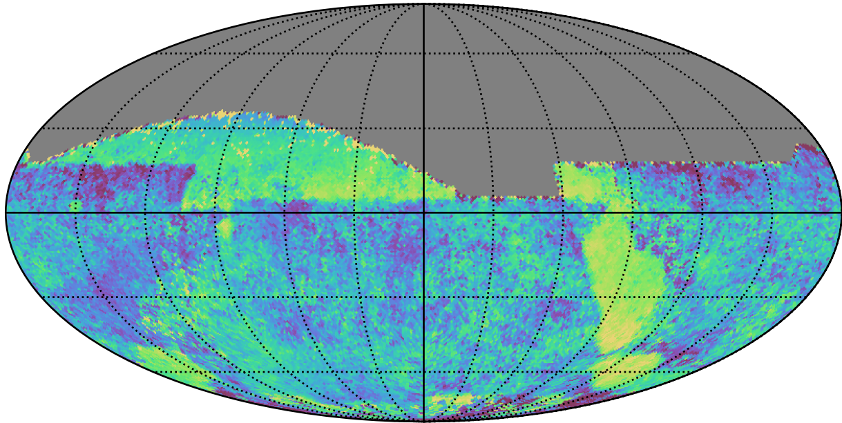
baseline_v3.0_10yrs All sky all bands: Median skyBrightness
