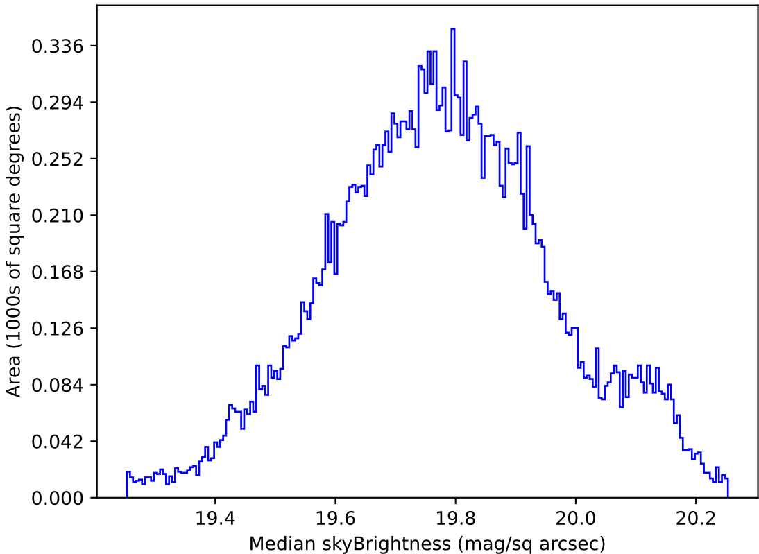
baseline_v3.0_10yrs All sky all bands: Median skyBrightness
