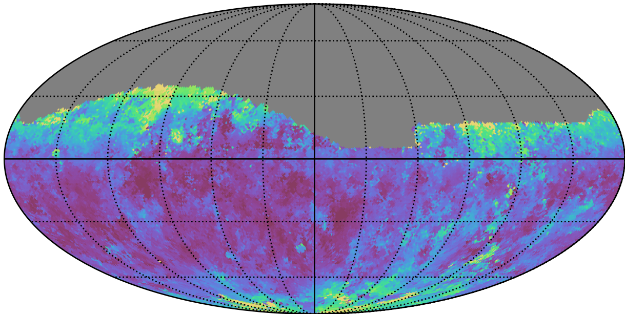
baseline_v3.0_10yrs Yr 1 z band: Median seeingGeom
