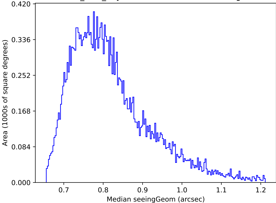
baseline_v3.0_10yrs Yr 1 z band: Median seeingGeom
