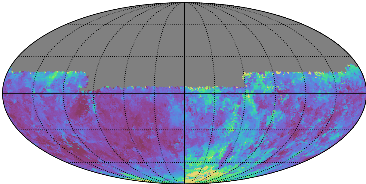
baseline_v3.0_10yrs Yr 1 y band: Median seeingGeom
