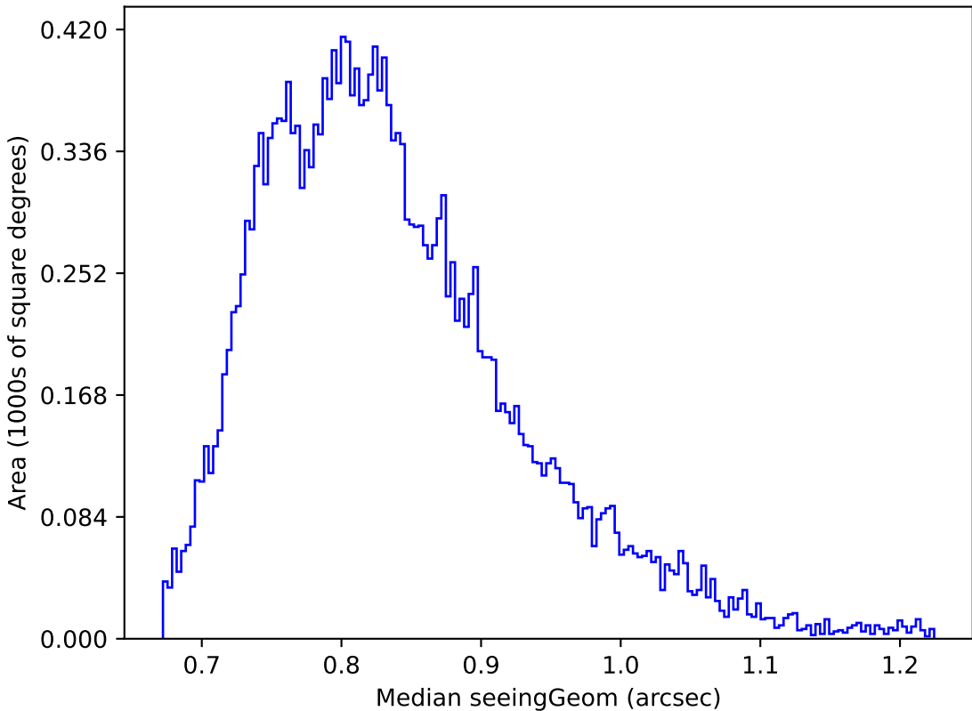
baseline_v3.0_10yrs Yr 1 y band: Median seeingGeom
