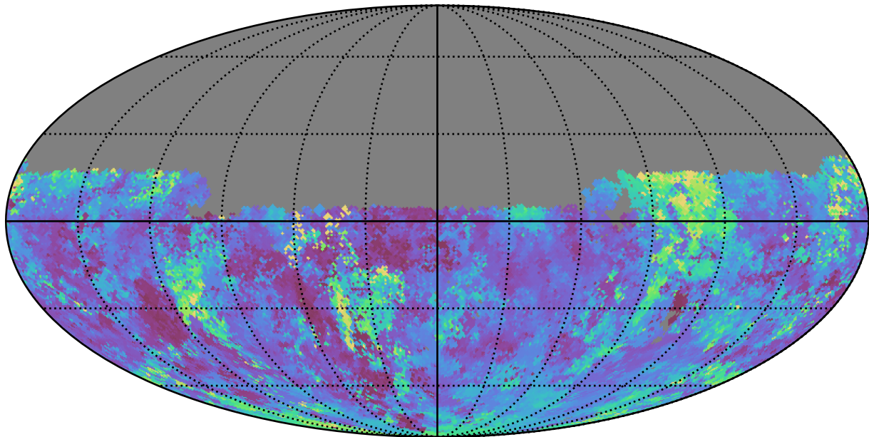
baseline_v3.0_10yrs Yr 1 u band: Median seeingGeom
