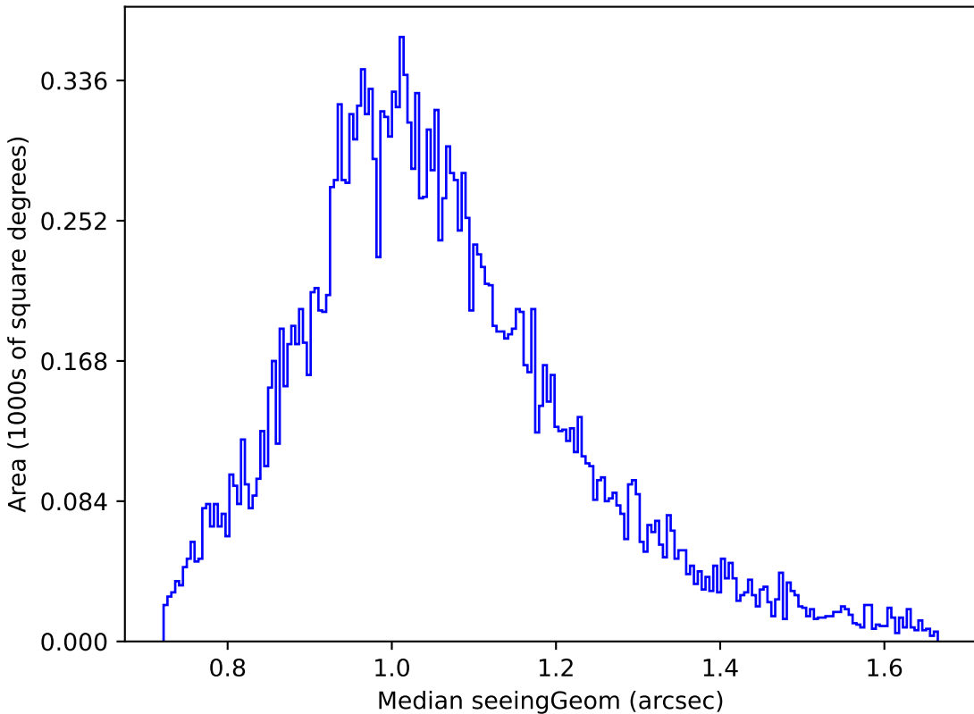
baseline_v3.0_10yrs Yr 1 u band: Median seeingGeom
