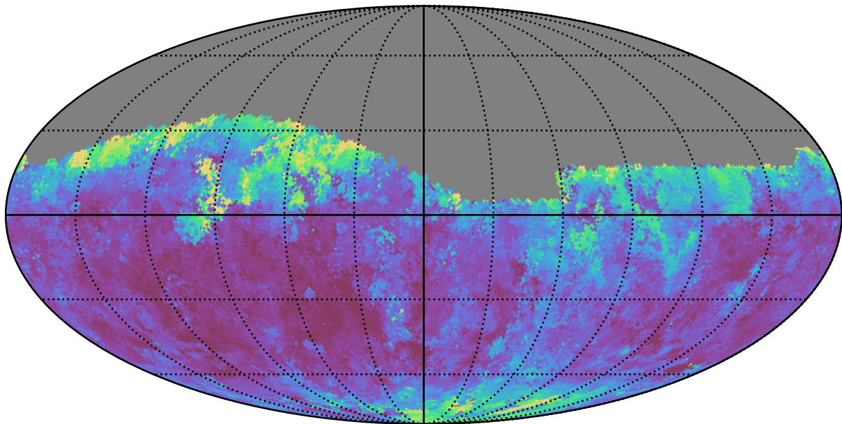
baseline_v3.0_10yrs Yr 1 r band: Median seeingGeom
