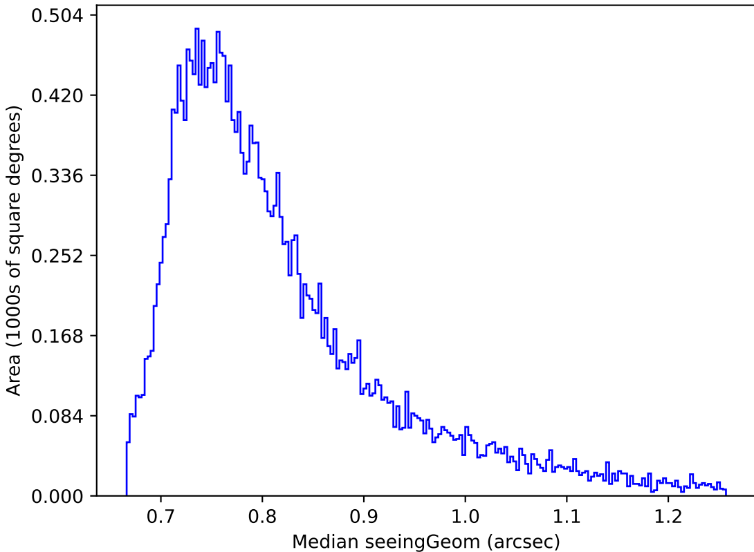
baseline_v3.0_10yrs Yr 1 i band: Median seeingGeom
