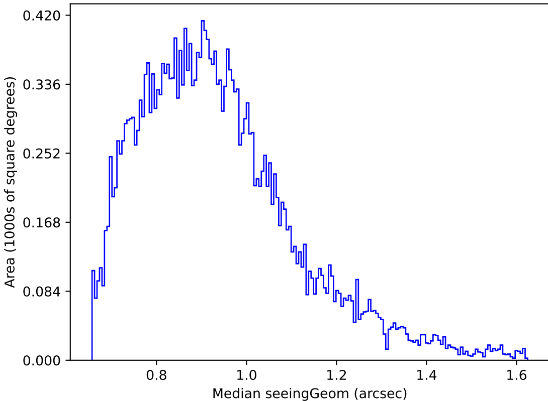
baseline_v3.0_10yrs Yr 1 g band: Median seeingGeom
