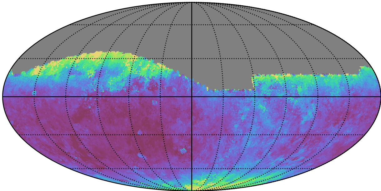
baseline_v3.0_10yrs Yr 1 all bands: Median seeingGeom
