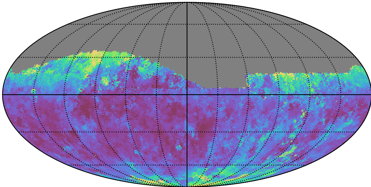
baseline_v3.0_10yrs Yr 1 z band: Median seeingEff
