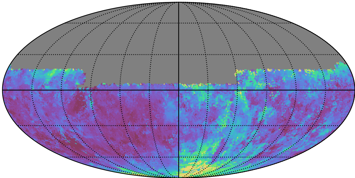
baseline_v3.0_10yrs Yr 1 y band: Median seeingEff
