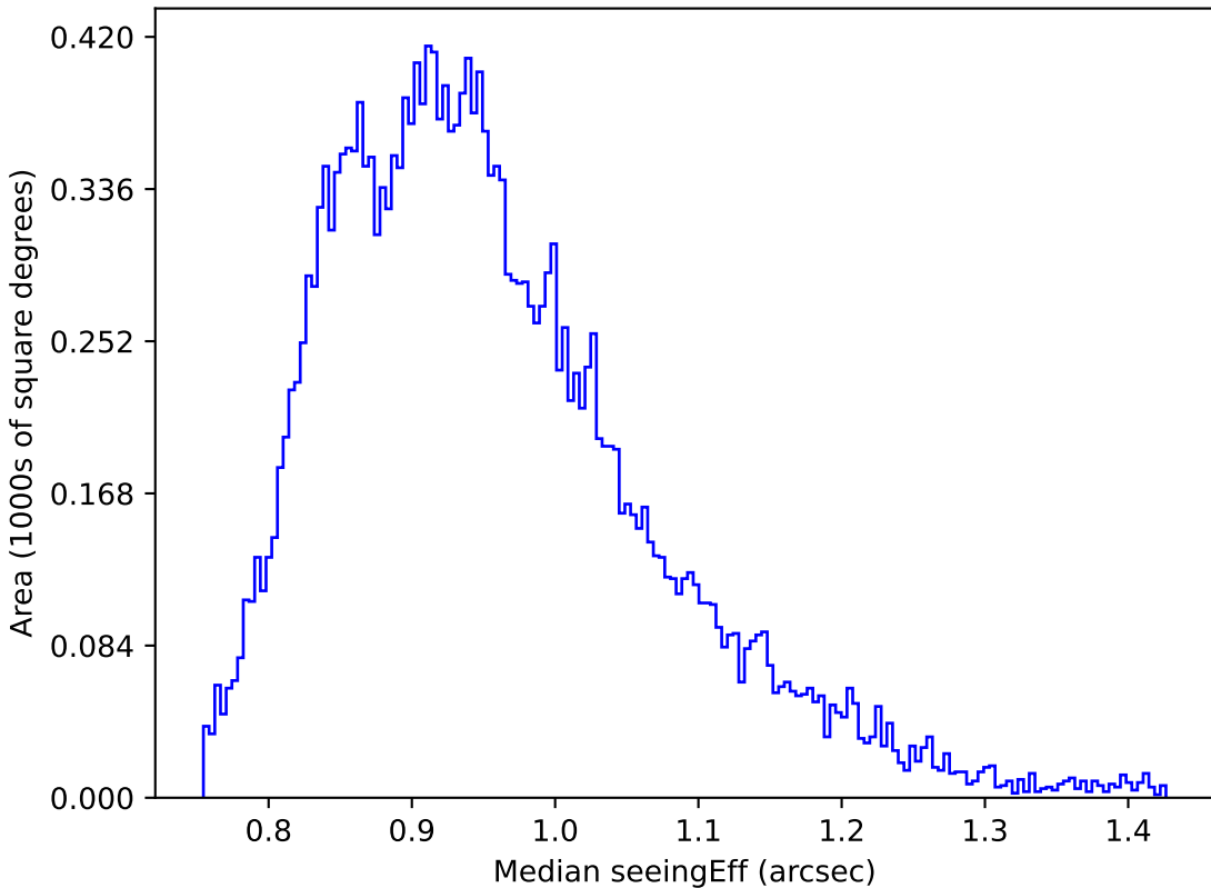
baseline_v3.0_10yrs Yr 1 y band: Median seeingEff
