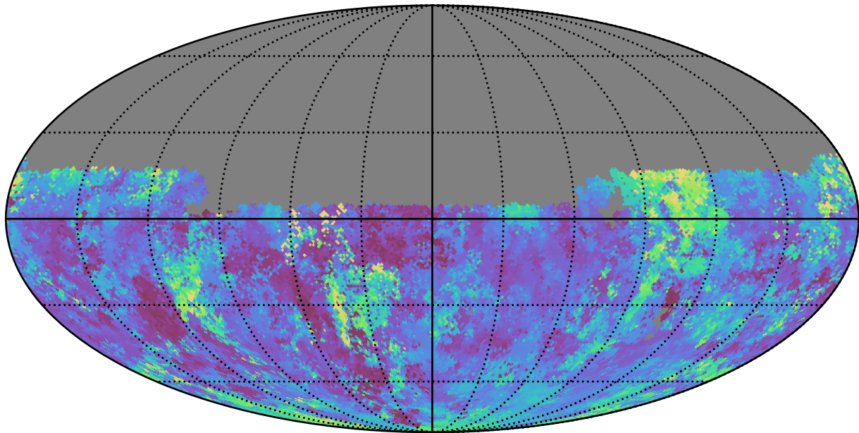
baseline_v3.0_10yrs Yr 1 u band: Median seeingEff
