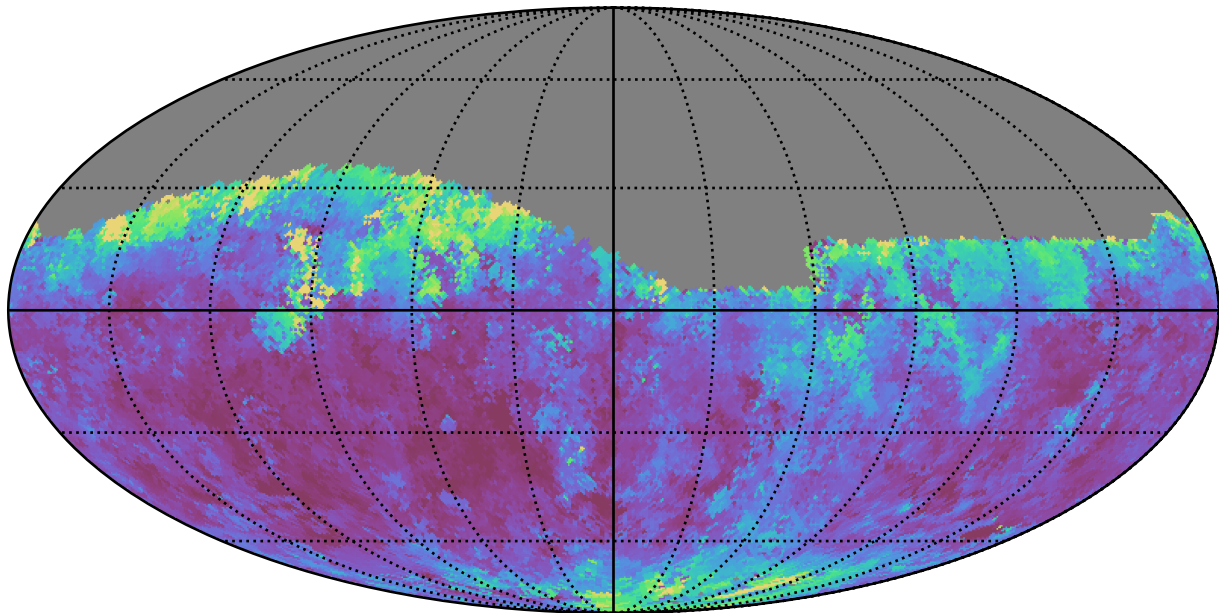
baseline_v3.0_10yrs Yr 1 r band: Median seeingEff
