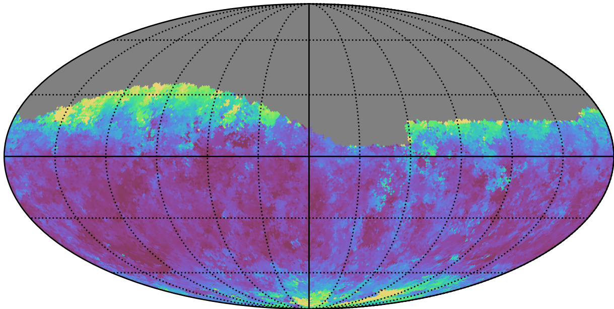
baseline_v3.0_10yrs Yr 1 i band: Median seeingEff
