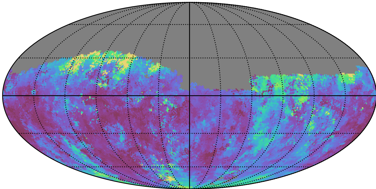
baseline_v3.0_10yrs Yr 1 g band: Median seeingEff
