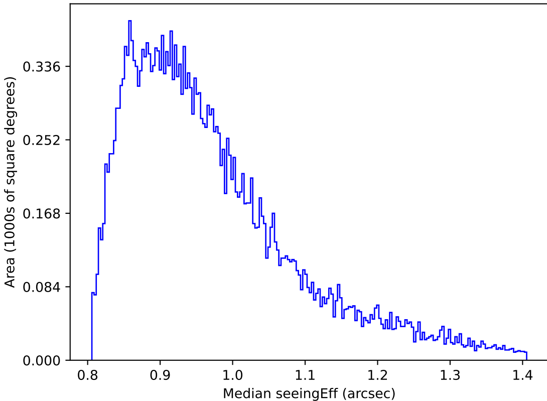
baseline_v3.0_10yrs Yr 1 all bands: Median seeingEff
