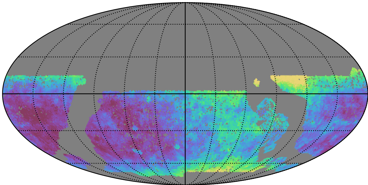
baseline_v3.0_10yrs WFD z band: Median seeingEff
