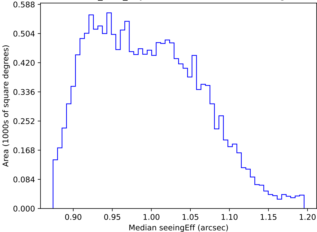
baseline_v3.0_10yrs WFD z band: Median seeingEff
