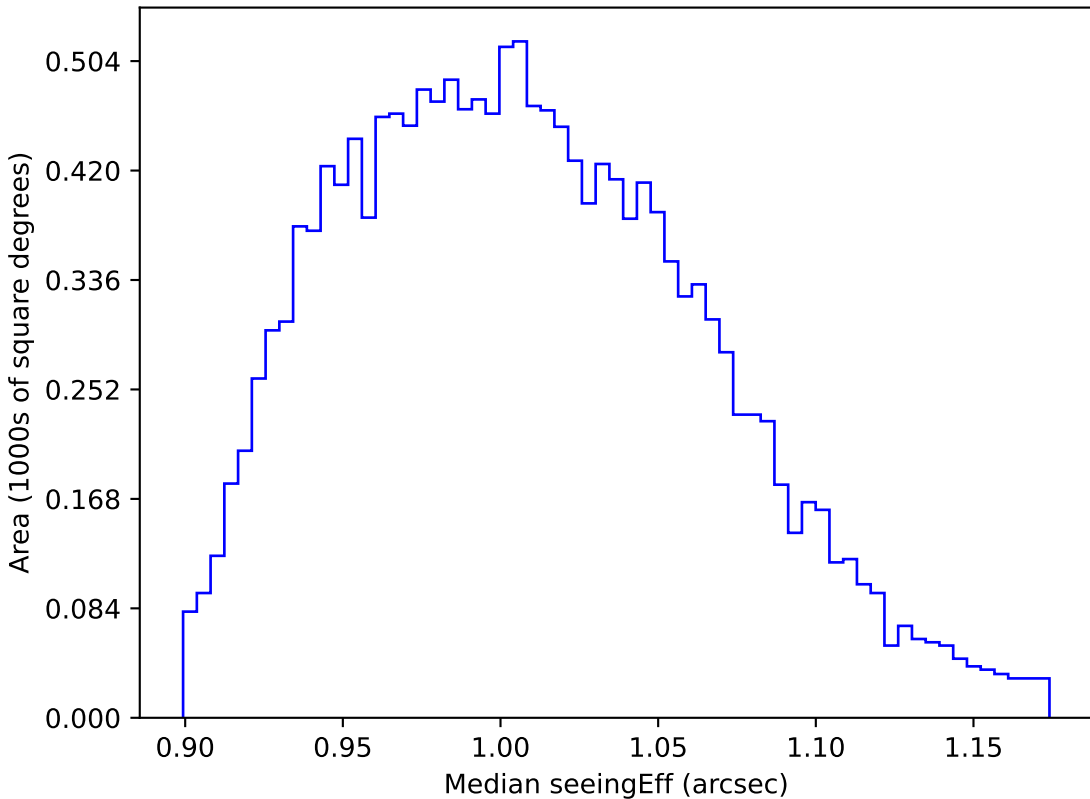
baseline_v3.0_10yrs WFD y band: Median seeingEff
