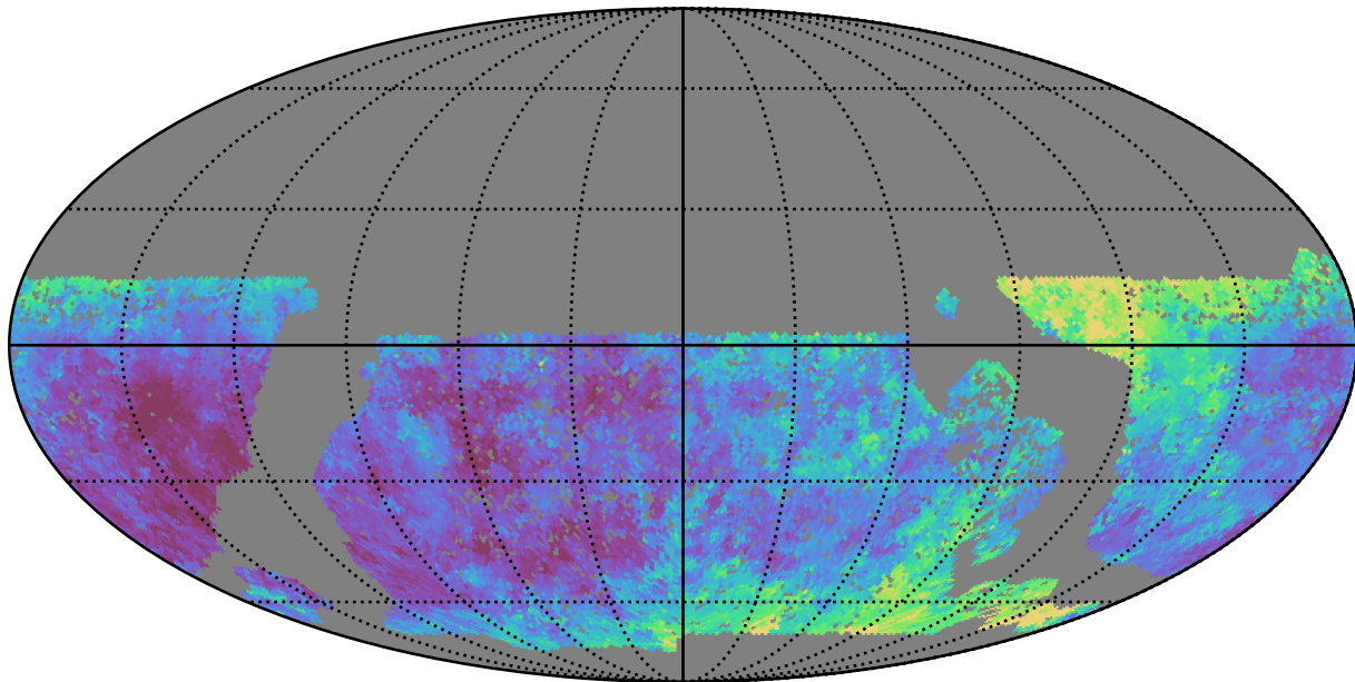
baseline_v3.0_10yrs WFD u band: Median seeingEff
