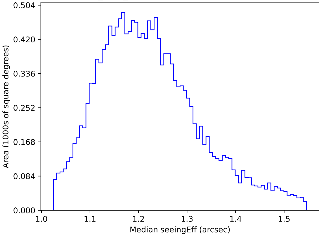
baseline_v3.0_10yrs WFD u band: Median seeingEff
