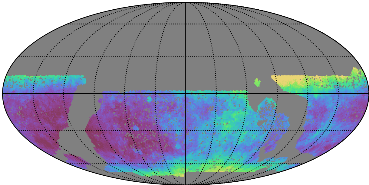
baseline_v3.0_10yrs WFD r band: Median seeingEff
