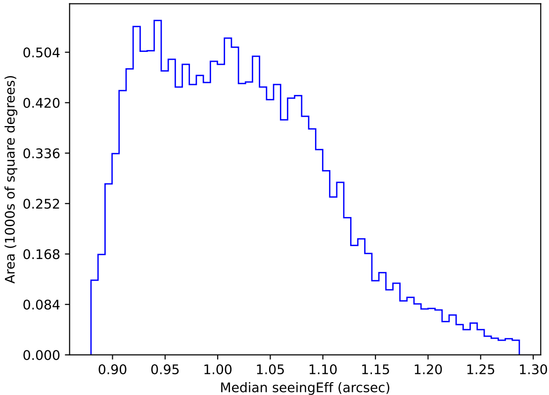
baseline_v3.0_10yrs WFD r band: Median seeingEff
