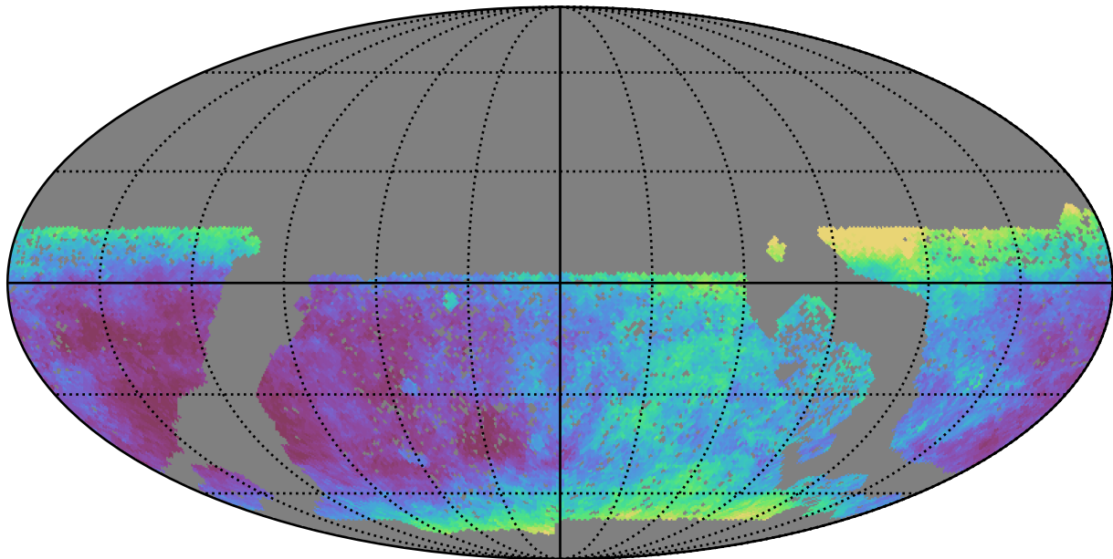
baseline_v3.0_10yrs WFD i band: Median seeingEff
