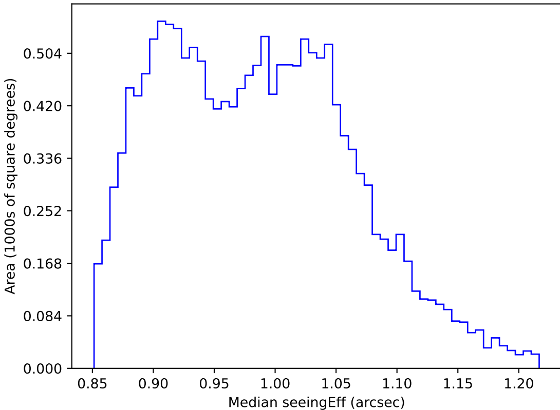
baseline_v3.0_10yrs WFD i band: Median seeingEff
