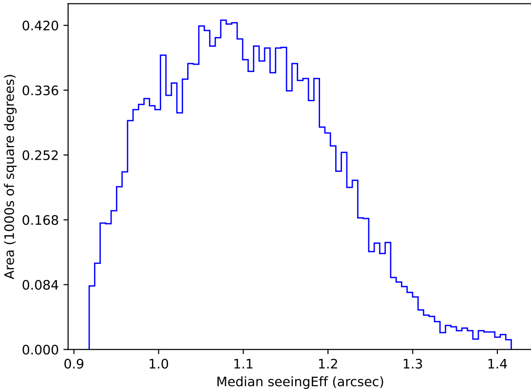
baseline_v3.0_10yrs WFD g band: Median seeingEff
