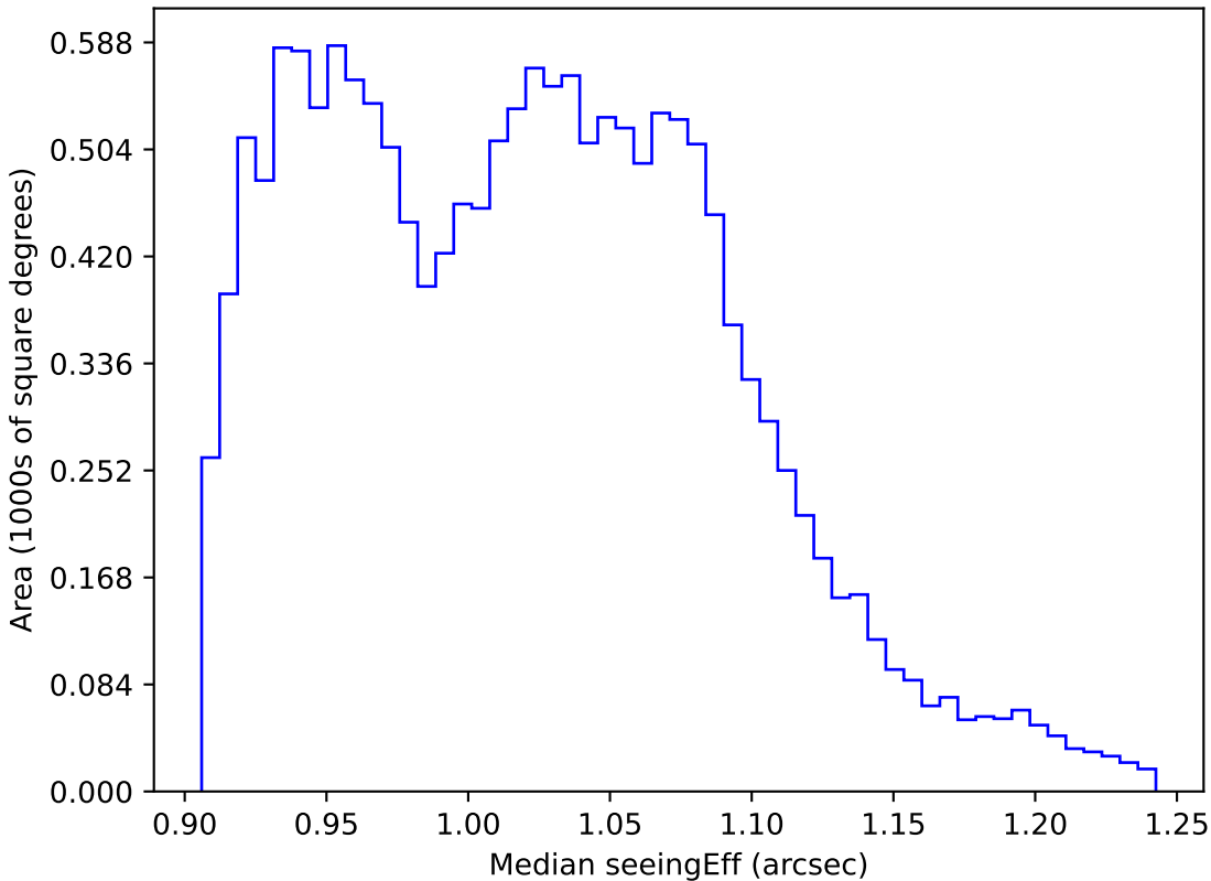
baseline_v3.0_10yrs WFD all bands: Median seeingEff
