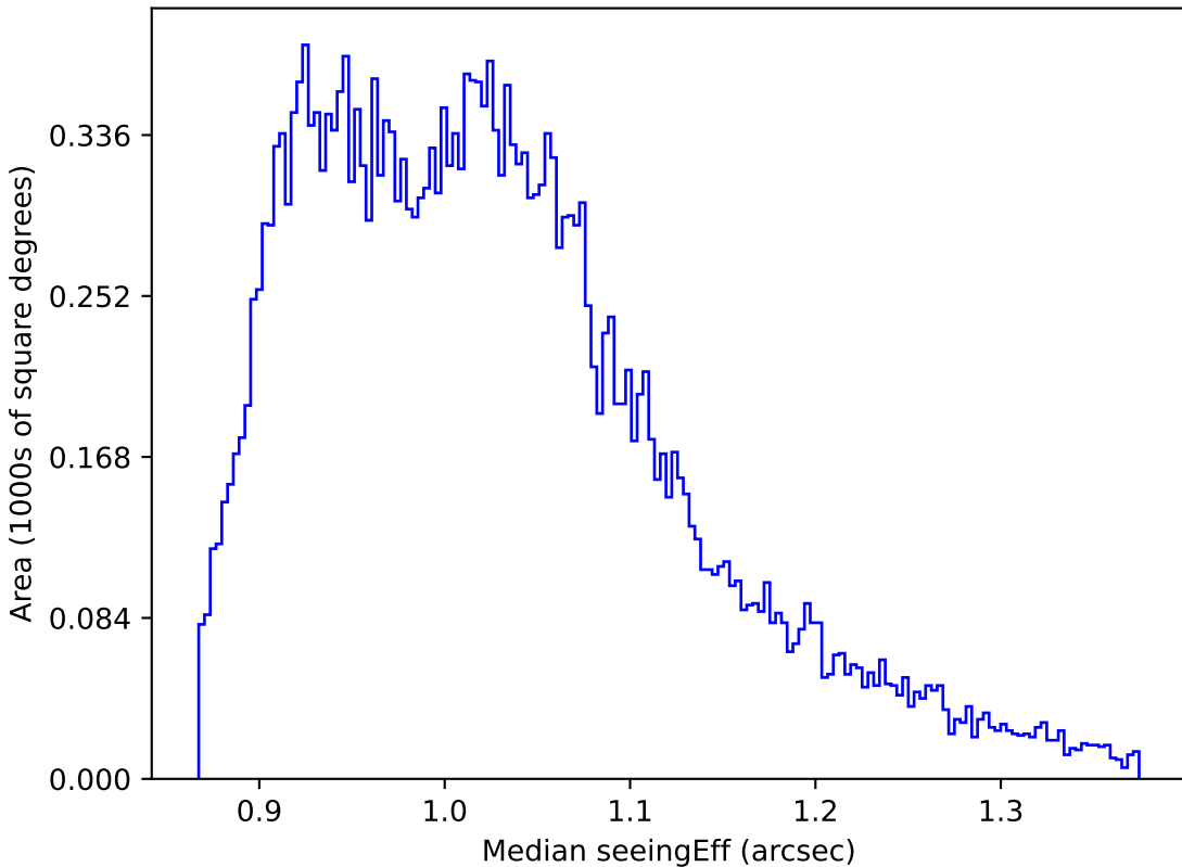
baseline_v3.0_10yrs All sky z band: Median seeingEff
