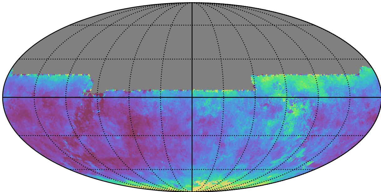
baseline_v3.0_10yrs All sky y band: Median seeingEff
