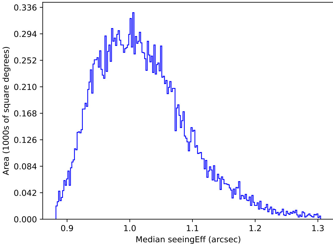
baseline_v3.0_10yrs All sky y band: Median seeingEff
