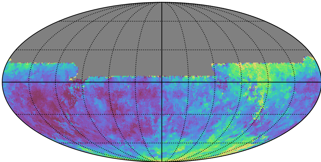
baseline_v3.0_10yrs All sky u band: Median seeingEff
