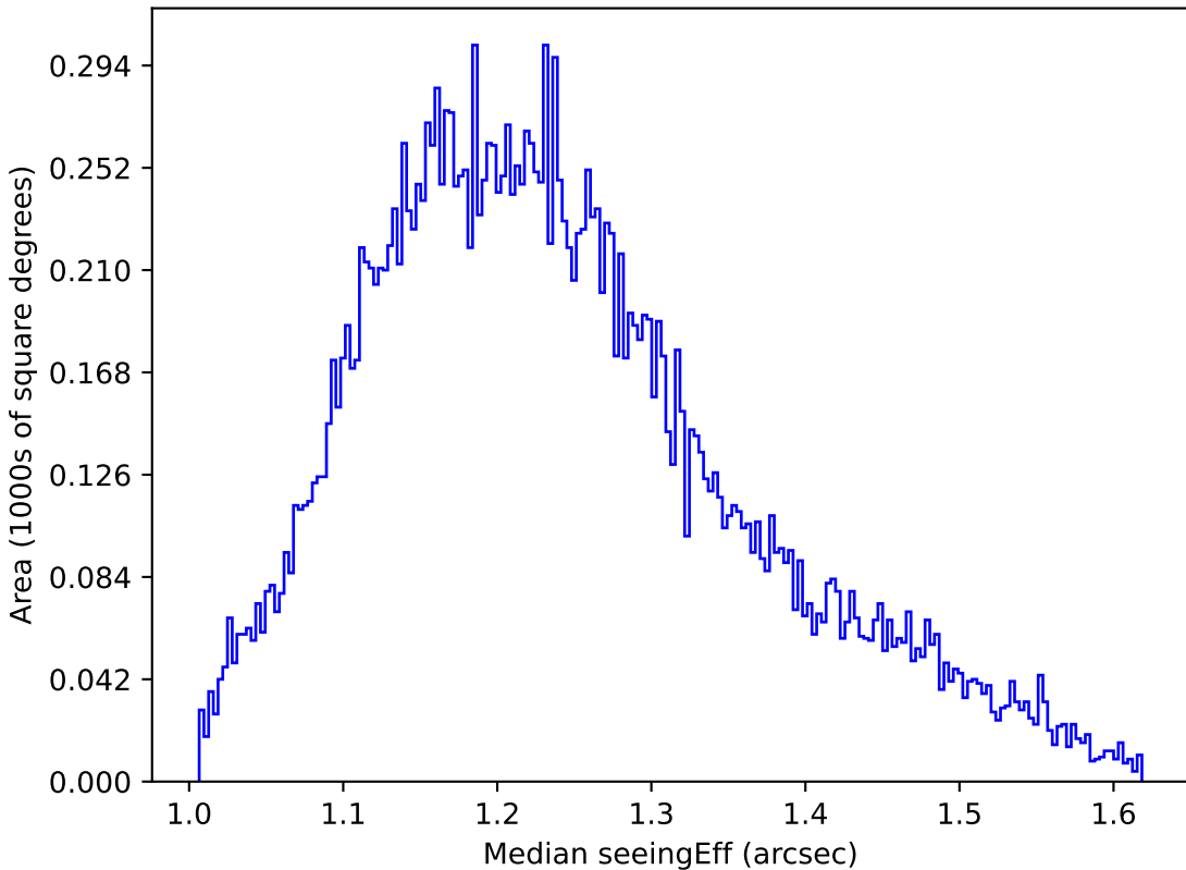
baseline_v3.0_10yrs All sky u band: Median seeingEff
