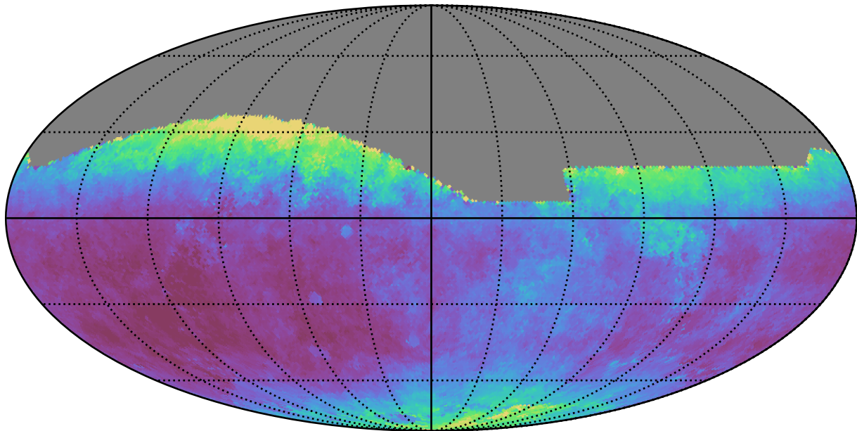
baseline_v3.0_10yrs All sky r band: Median seeingEff
