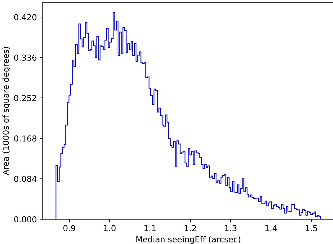
baseline_v3.0_10yrs All sky r band: Median seeingEff
