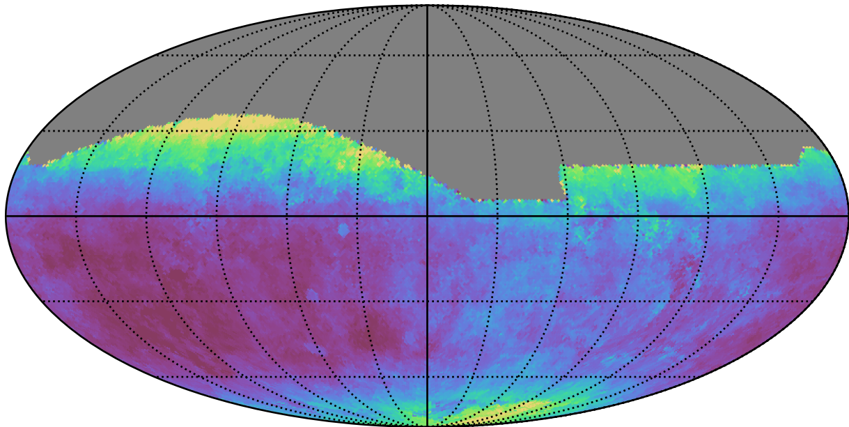
baseline_v3.0_10yrs All sky i band: Median seeingEff
